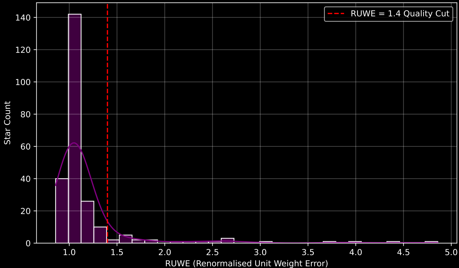
GALAH DR4 Field [2955] RUWE Distribution (n= 241)
