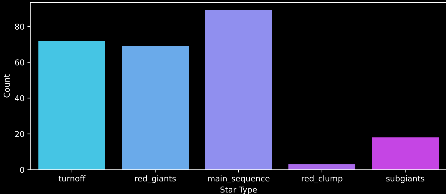
GALAH DR4 Field: [2955] Count plot of Star Type
